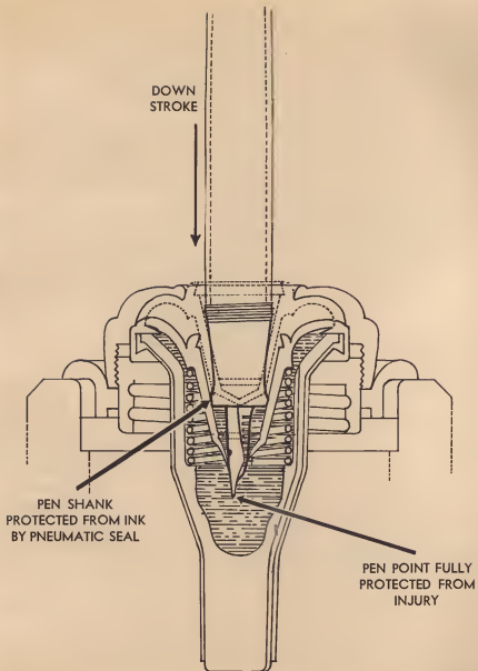
SECOND — Compression Stroke (Gently Pressed Down About \frac{1}{4} Inch)
